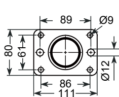
Rectangular plate
