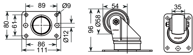
Rectangular plate
