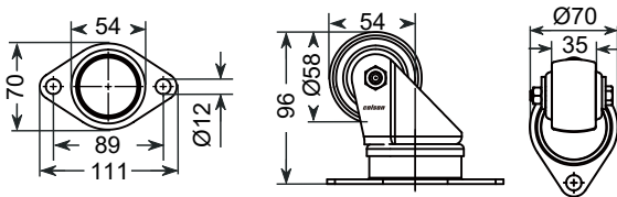
Diamond plate
