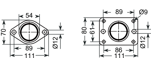
Diamond plate
