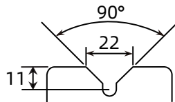
V-groove cast iron wheel width and depth dimensions
