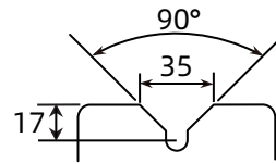
10 inches V-groove cast iron wheel width and depth dimensions
