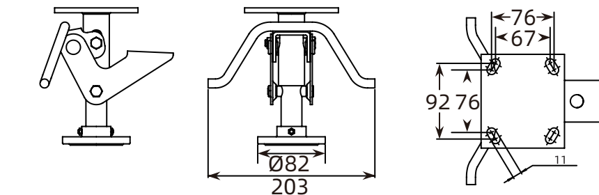
-4、6 series Installation size chart
