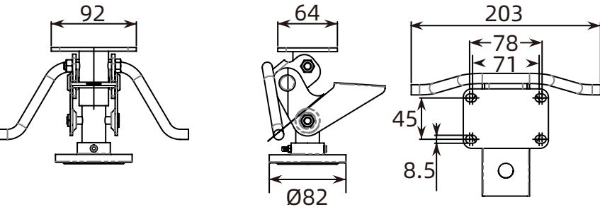
-4、6 series Installation size chart
