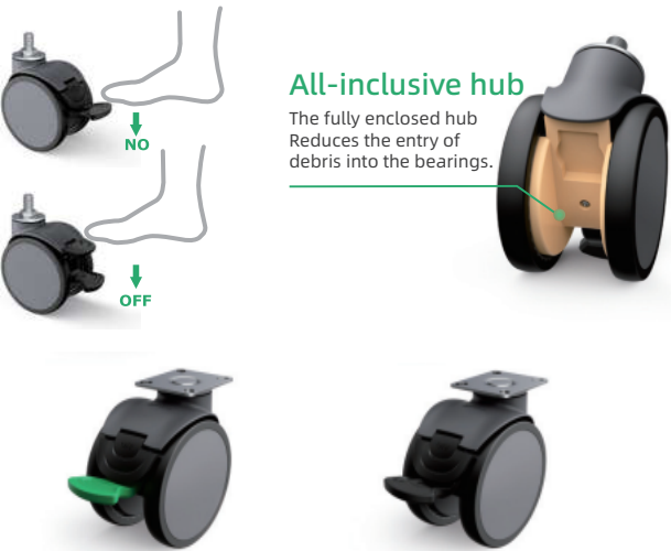
Direction Lock9 (DL) Total Lock (BRK4)
