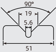
V-groove cast iron wheel width and depth dimensions
