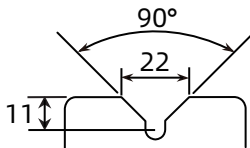
V-groove cast iron wheel width and depth dimensions
