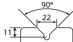
8 inches V-groove cast iron wheel width and depth dimensions
