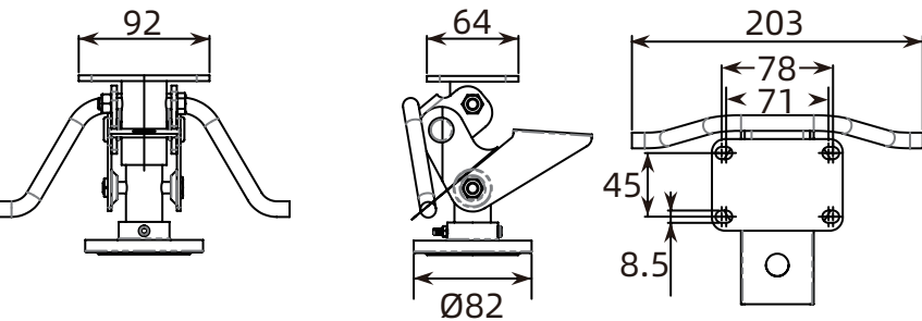
-4、6 series Installation size chart
