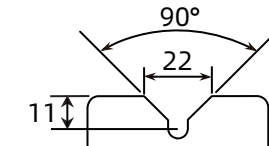
8 inches V-groove cast iron wheel width and depth dimensions
